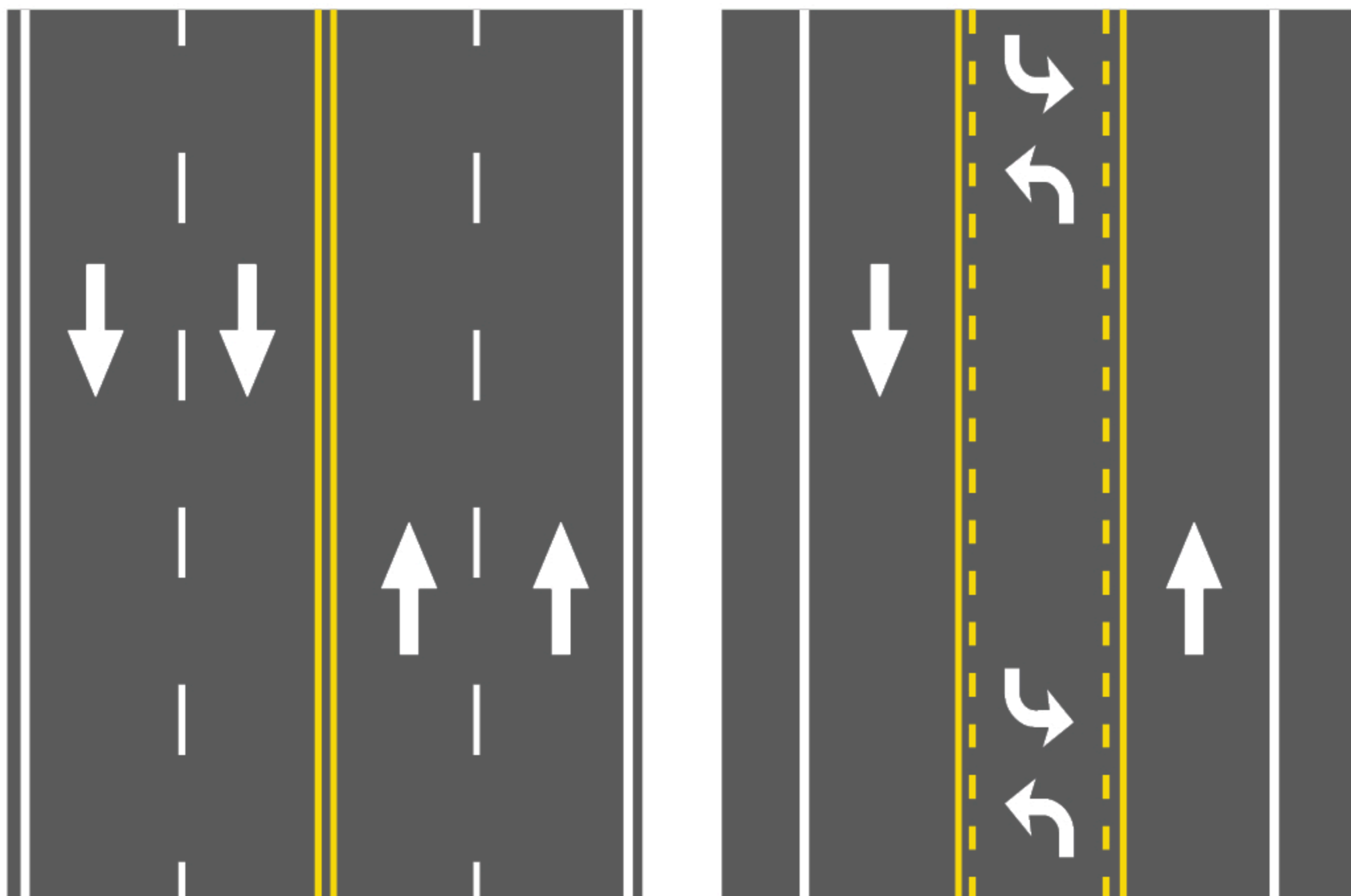
Figure 1. Road Diet Example
